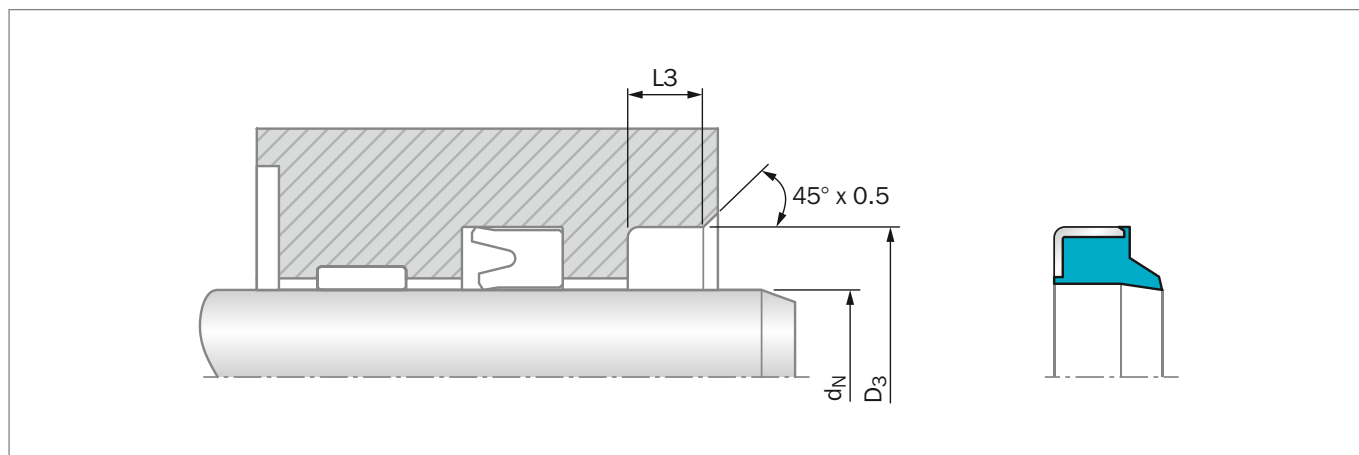
Figure 212: Installation Drawing
