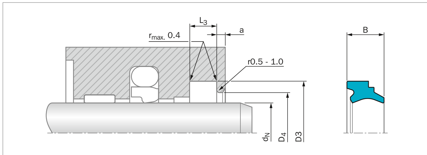
Figure 197: Installation Drawing
