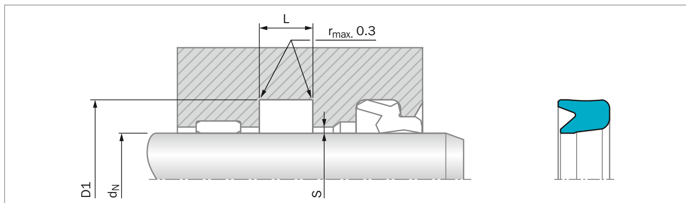
Figure 68: Installation Drawing, Dimension "S" see Figure 67
