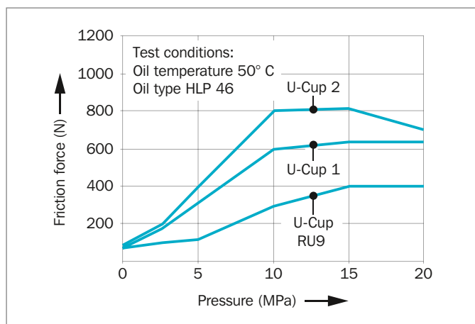
Figure 63: Friction dependent on pressure
