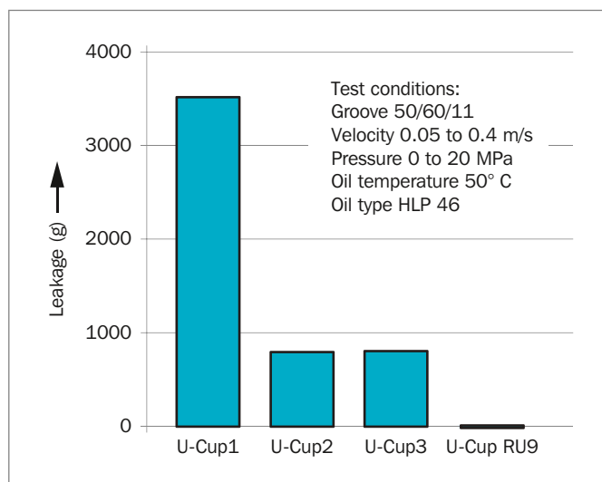
Figure 66: Leakage performance dependent on U-Cup type
