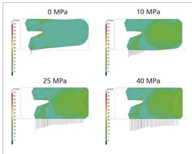
Figure 65: How the Zurcon® U-Cup RU9 performs underpressure
