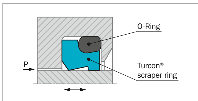
Figure 175: Turcon® Excluder® 5
