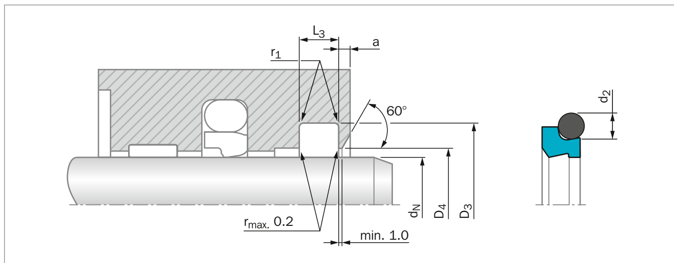
Figure 176: Installation Drawing
