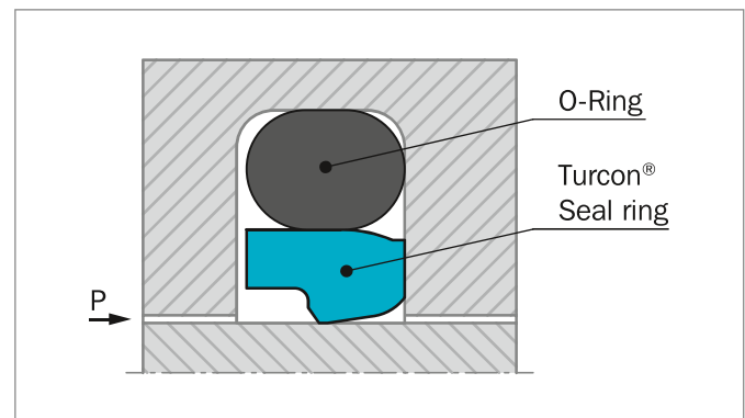
Figure 17: Turcon® Stepseal® 2K
